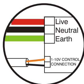
Connections to 1-10v HF dimmable ballast (example only)
