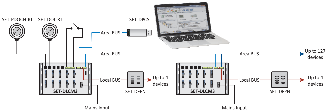
Figure 1. Wiring.
