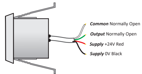
Figure 2. Wiring
