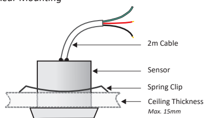
Figure 1. Rear Mounting
