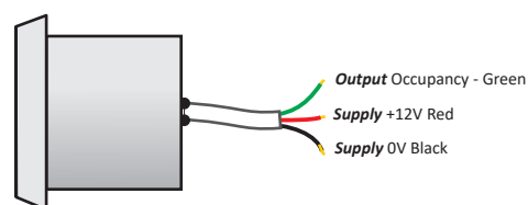
Figure 2. Wiring
